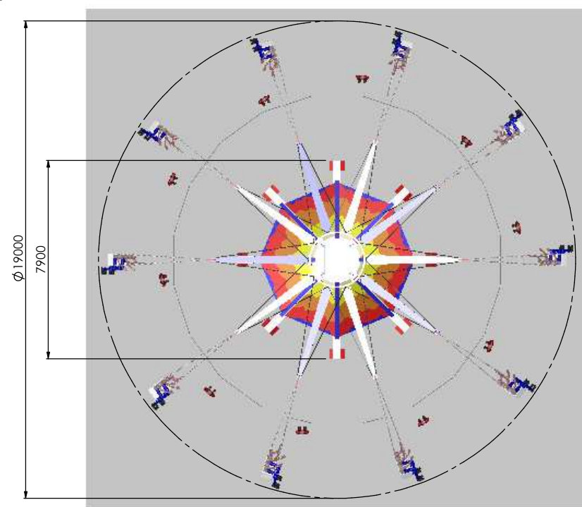
TOP VIEW IN OPERATION
